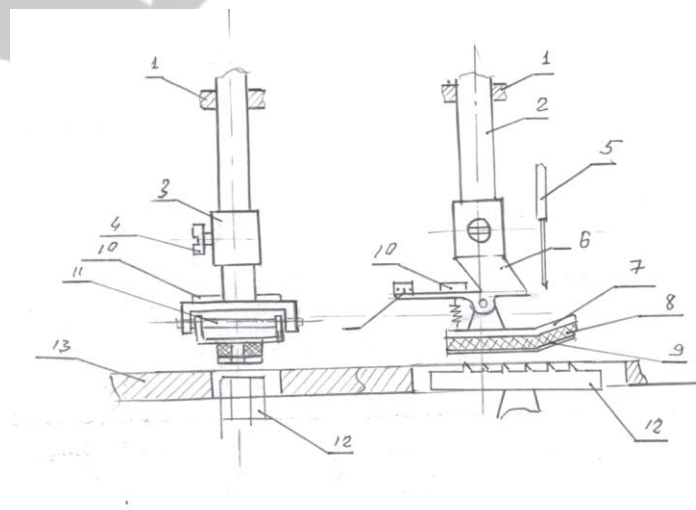
Fig.2. Scheme of the paws installed on the stand with strain gauge sensors for controlling the load on the paws
