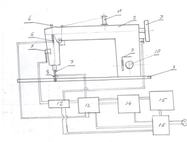
a - General view of the experimental setup of the sewing machine with the proposed paws design.
